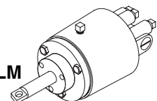
TRADITIONAL TILT (available for all SeaStar 1.7, 2.4 & SeaStar PRO systems, not Capilano & Hynautic)
