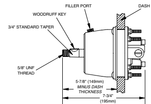
HA5418 BACK PLATE KIT
